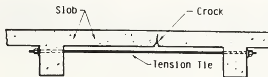
a) To Correct Cracking of Slob
